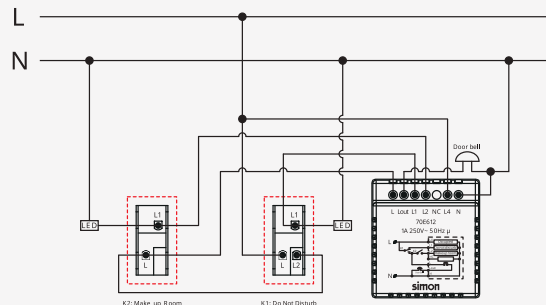
LED on when loads connected
